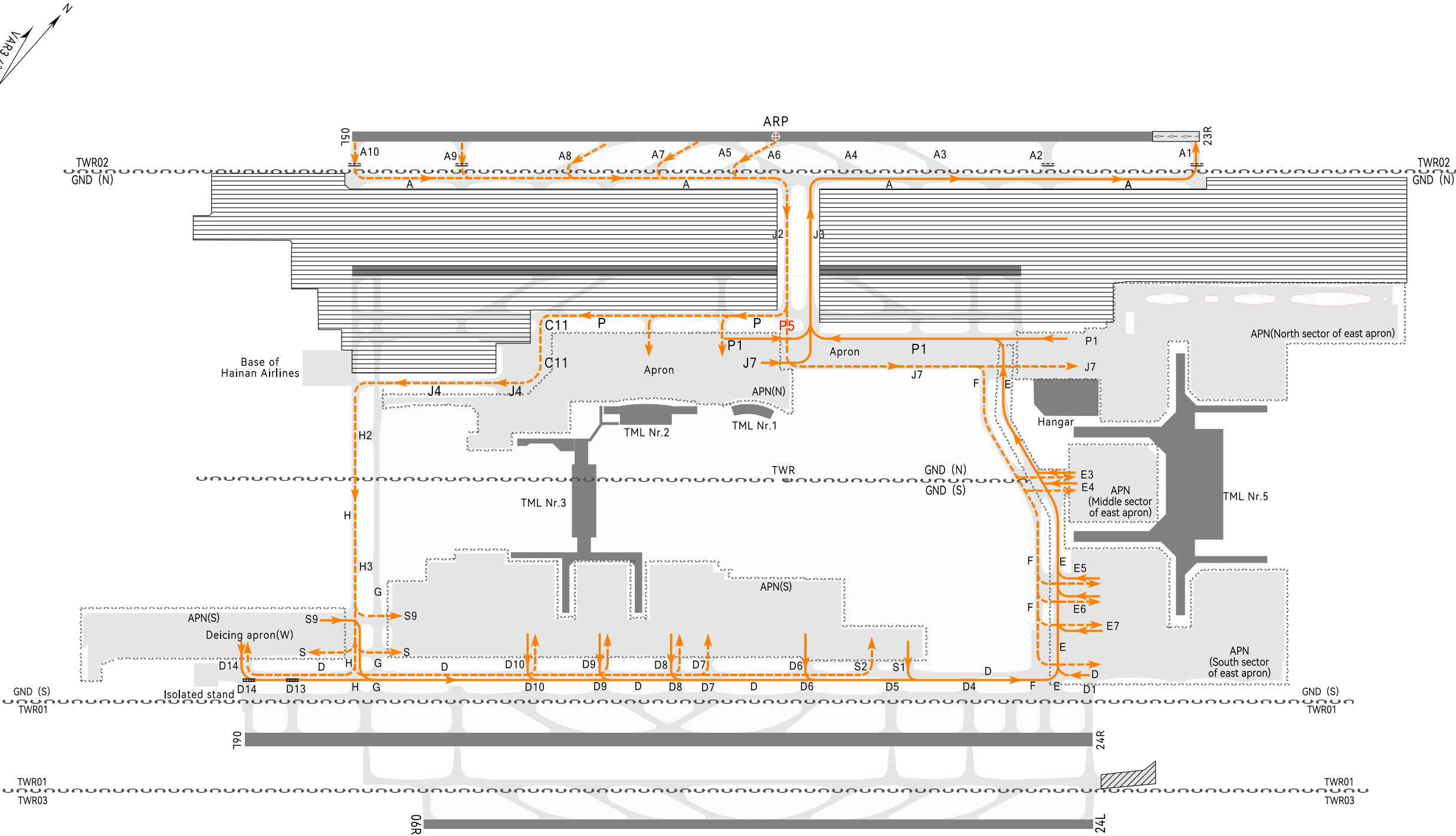
Taxiing Routes Chart RWY23R
